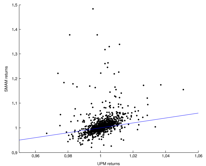
Fig. 5.1. SMAM returns vs UPM returns: the returns on the portfolio constructed from the semiparametric model average method are on the vertical axis and those on the portfolio constructed from the unconditional parametric method are on the horizontal axis; the straight line is y = x .
